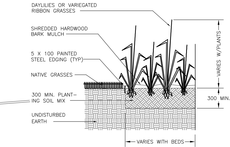
GROUNDCOVER BED PLANTING DETAIL N.T.S.
