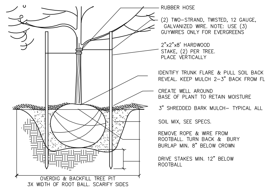
TREE PLANTING & STAKING NOT TO SCALE
