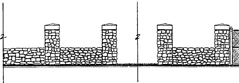
Optional Stone Pier Treatment meeting Chain Link Fence and Stone Wall
