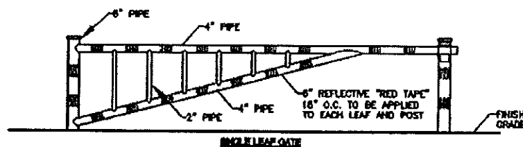
Vehicular Entrance Gates Detail
