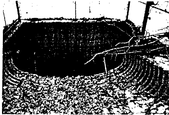
Vertical shaft opening in culvert structure E, 1998, needs protective grate.
