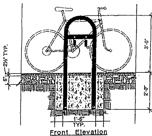
Bicycle Rack Detail
