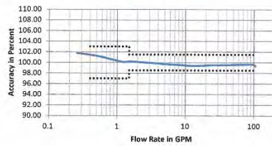
Rate of Flow in Gallons per Minute (gpm) 1-1/2" Meter
